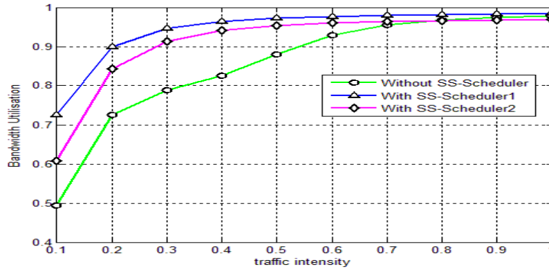
Figure 7. Bandwidth Utilization of the system
