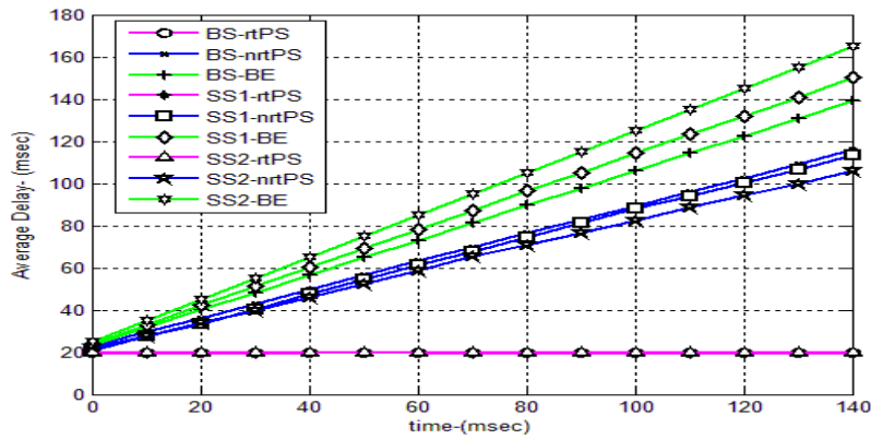
Figure 2. Service delay comparison
