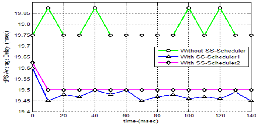
Figure 3. Service delay comparison of rtPS
