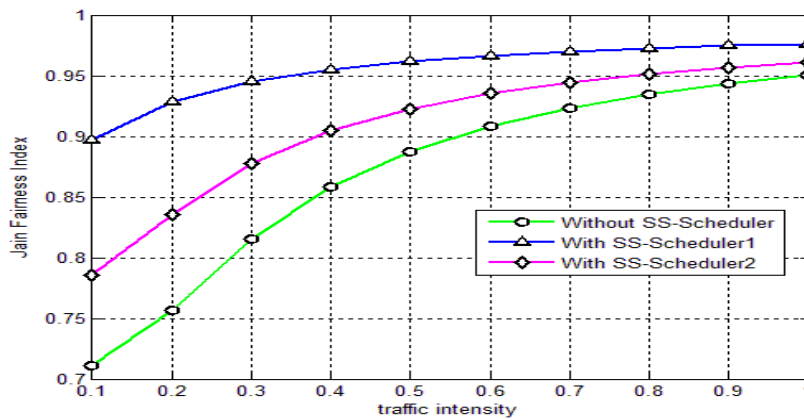
Figure 8. Jain's Fairness Index
