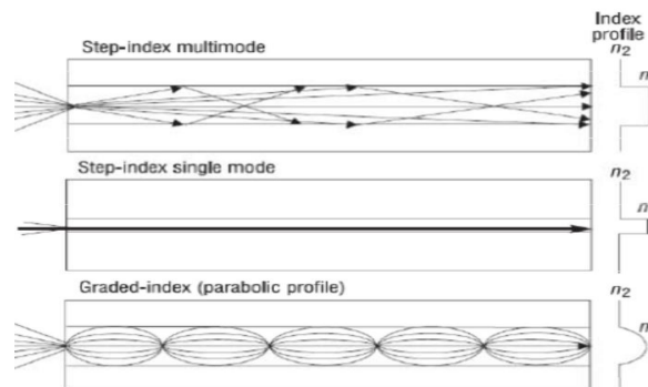
Figure 2 gives a description of the various optical fiber modes.
