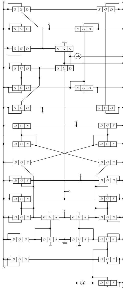
Fig. 1a. Structure of considered current follower transconductance amplifier [18]
