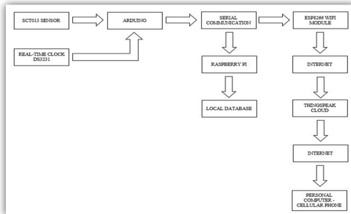
Figure 2. Block Diagram
