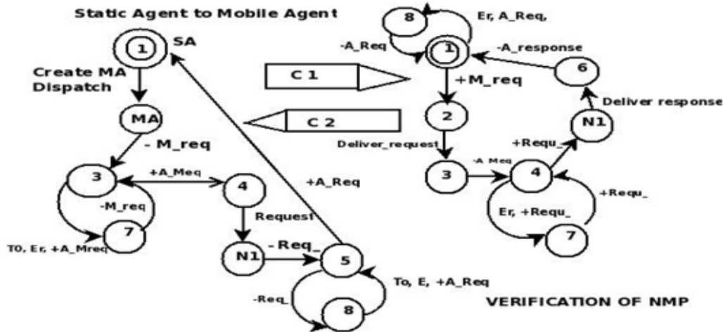
Figure 3: Verification of NMP
