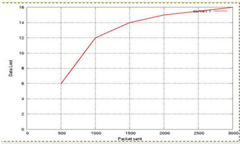
Figure 16: Data loss verses number of packets sent
