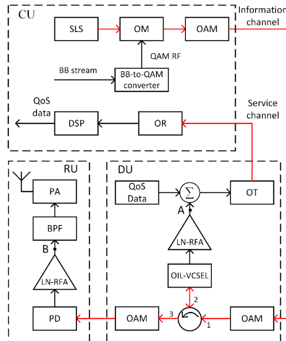
Figure 2. Block-diagram of the proposed duplex communication channel for NG-RAN, where SLS, OM, OAM, DSP, OR, OT, PD, LN-RFA, BPF, and PA stand for semiconductor laser source, optical modulator, optical amplifier, digital signal processor, optical receiver, optical transmitter, photodetector, low-noise RF amplifier, bandpass RF filter, and power RF amplifier (Optical connections are painted in red, electrical connections – in black)
