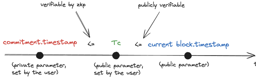
Fig. 1. Verifiable commitment timestamp rules
