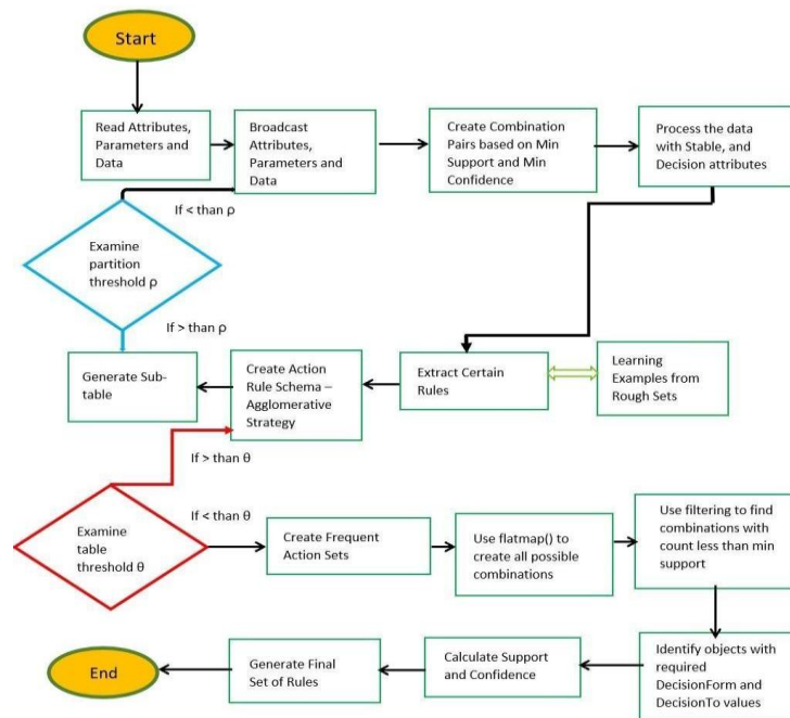
Figure 2. Hybrid Action Rule Mining Algorithm (New Threshold) – Flowchart
