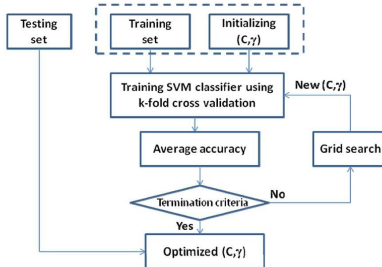
Figure 2: Flowchart selection for optimal parameters using grid search [25].
