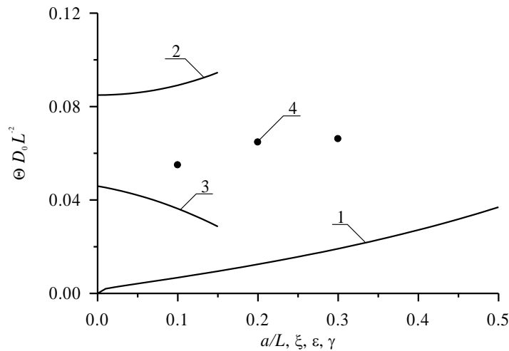
Fig.5b. Dimensionless optimal annealing time of implanted dopant as a function of several parameters. Curve 1 describes the dependence of the annealing time on the relation a/L and \xi=\gamma=0 for equal to each other values of dopant diffusion coefficient in all parts of heterostructure. Curve 2 describes the dependence of the annealing time on value of parameter \varepsilon for a/L=1/2 and \xi=\gamma=0 . Curve 3 describes the dependence of the annealing time on value of parameter \xi for a/L=1/2 and \varepsilon = \gamma=0 . Curve 4 describes the dependence of the annealing time on value of parameter \gamma for a/L=1/2 and \varepsilon=\xi=0
