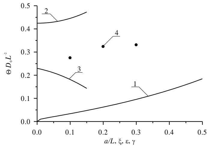
Fig. 5a. Dimensionless optimal annealing time of infused dopant as a function of several parameters. Curve 1 describes the dependence of the annealing time on the relation a/L and \xi=\gamma=0 for equal to each other values of dopant diffusion coefficient in all parts of heterostructure. Curve 2 describes the dependence of the annealing time on value of parameter \varepsilon for a/L=1/2 and \xi=\gamma=0 . Curve 3 describes the dependence of the annealing time on value of parameter \xi for a/L=1/2 and \varepsilon = \gamma=0 . Curve 4 describes the dependence of the annealing time on value of parameter \gamma for a/L=1/2 and \varepsilon=\xi=0
