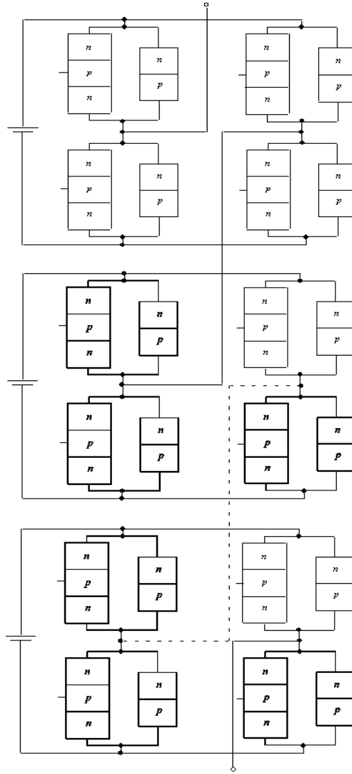
Fig. 1. The considered inverter
