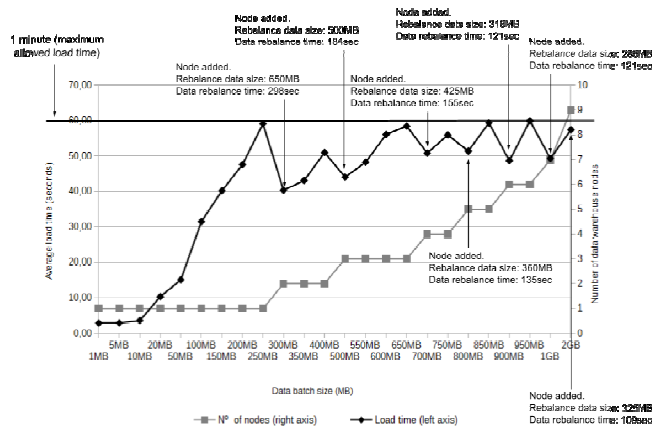
Figure 16: Data warehouse load scalability
