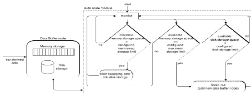
Figure 6: Data Buffers, scale-out
