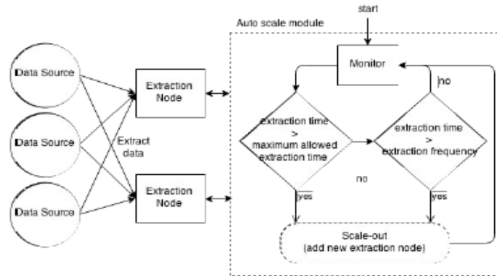
Figure 3: Extraction algorithm, scale-out
