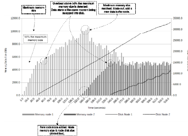
Figure 15: Data buffer swap into disk and scaling
