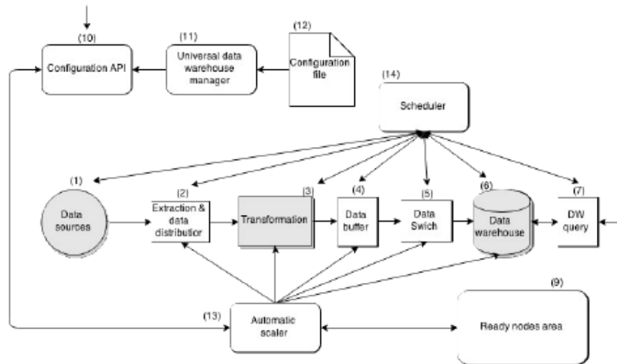
Figure 1: Automatic ETL+Q scalability
