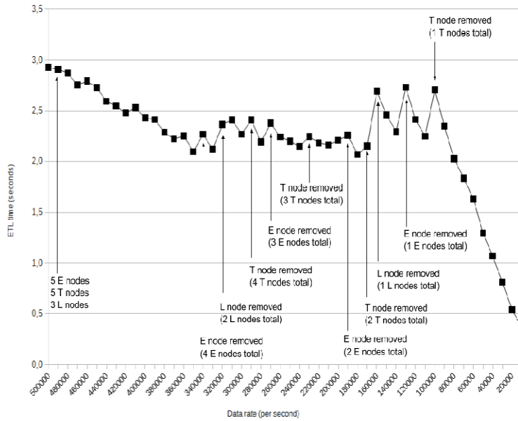
Figure 11: Full ETL system scale-in
