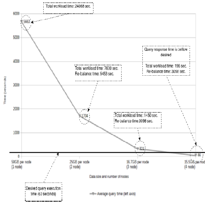
Figure 17: Data warehouse scalability, workload 1
