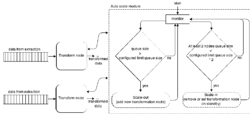
Figure 5: Transformation, scale-in and scale-out
