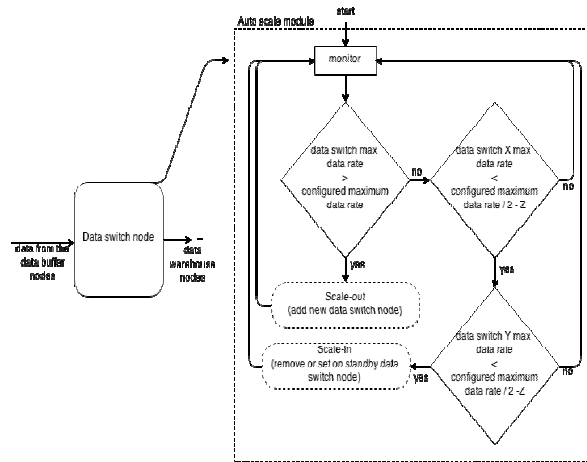
Figure 7: Data switch, scale
