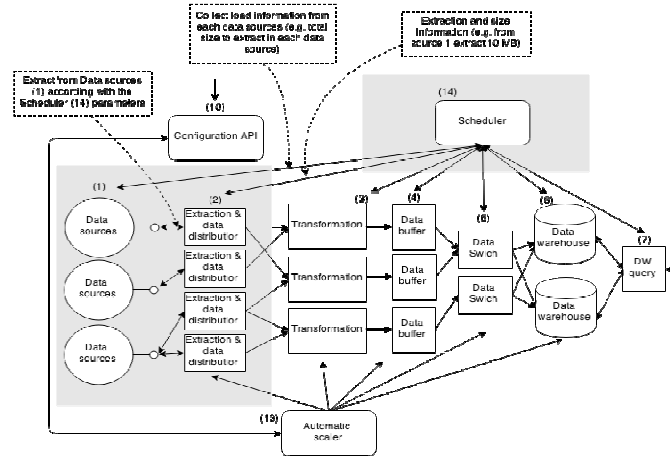
Figure 12: Sources to extraction
