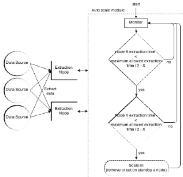
Figure 4: Extraction algorithm, scale-in
