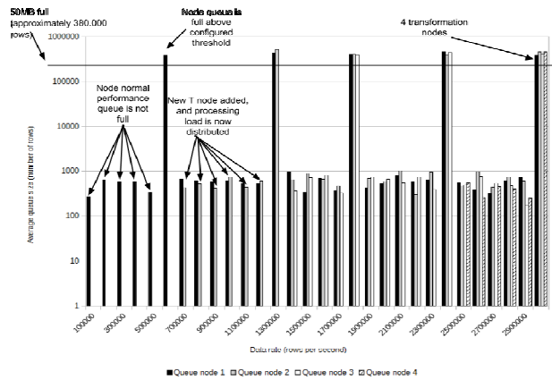
Figure 14: Automatic transformation scalability. 60 minutes processing per data-rate.
