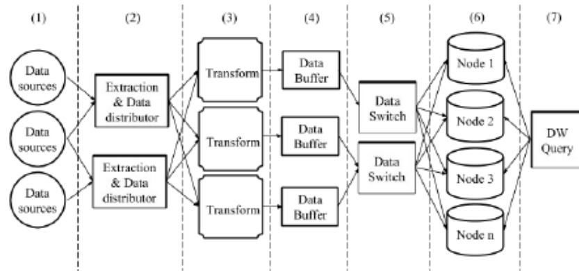
Figure 2: Total automatic ETL+Q scalability
