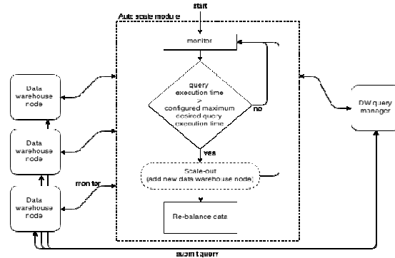
Figure 9: Data warehouse scale based on query time
