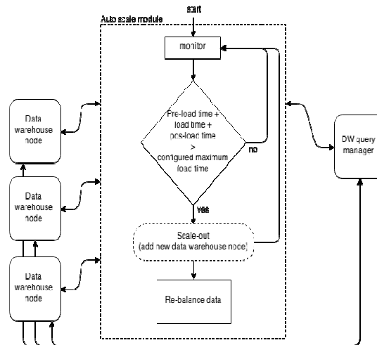
Figure 8: Data warehouse scale
