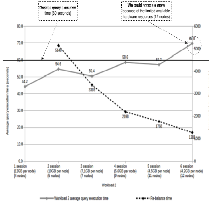
Figure 18: Data warehouse scalability, workload 2
