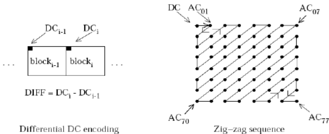
Fig 7: Preparation of Quantized Coefficients for Entropy Coding
