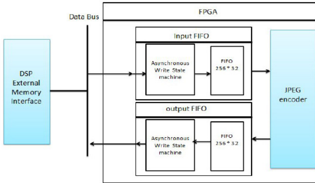
Fig 10: Two FIFO channels.
